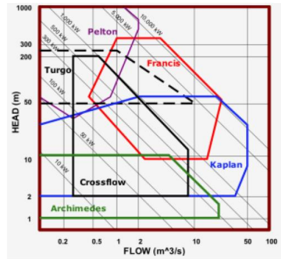
Figure 5-1 - Use of turbine types by head height, discharge, or capacity
