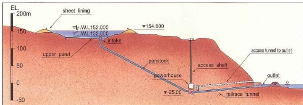
Figure 12-1: Okinawa Yambaru sea water pumped-storage plant. General view of the site and profile of waterways
