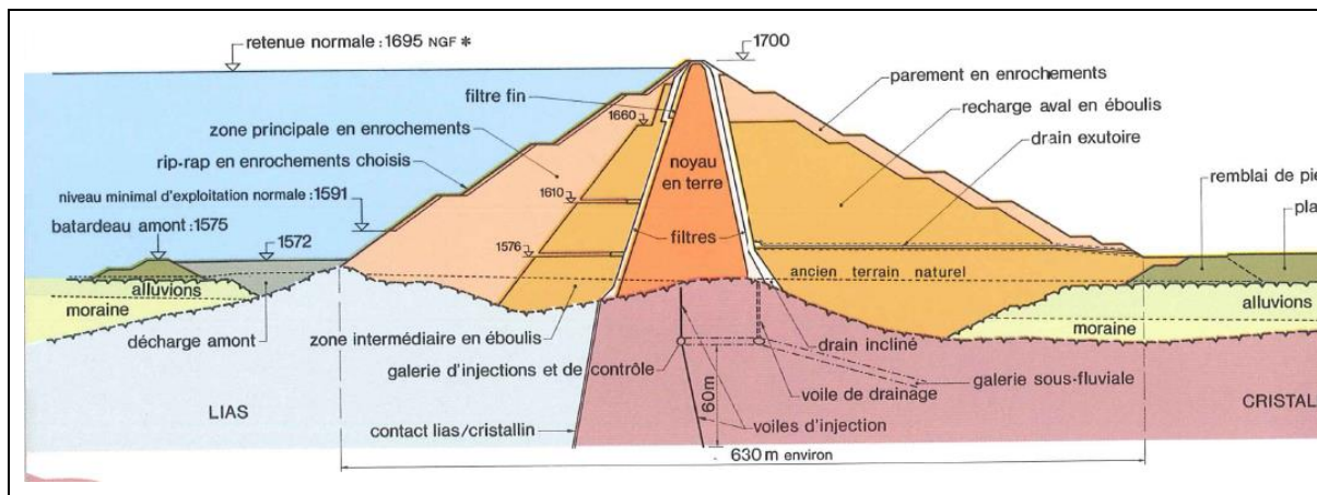
Figure 4-1 - Embankment dam with a core of impervious material (clay and silt)
