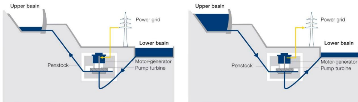
Figure 2-3 - Functioning of PSH in pumping and turbining mode (source: Voith)
