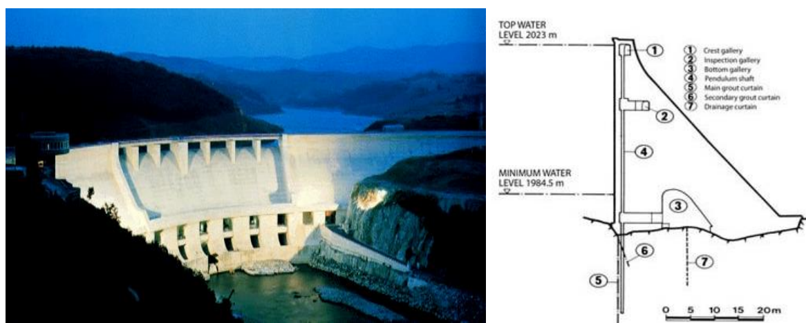
Figure 4-3: Villerest Gravity dam (left) and typical section of a gravity dam (right)
