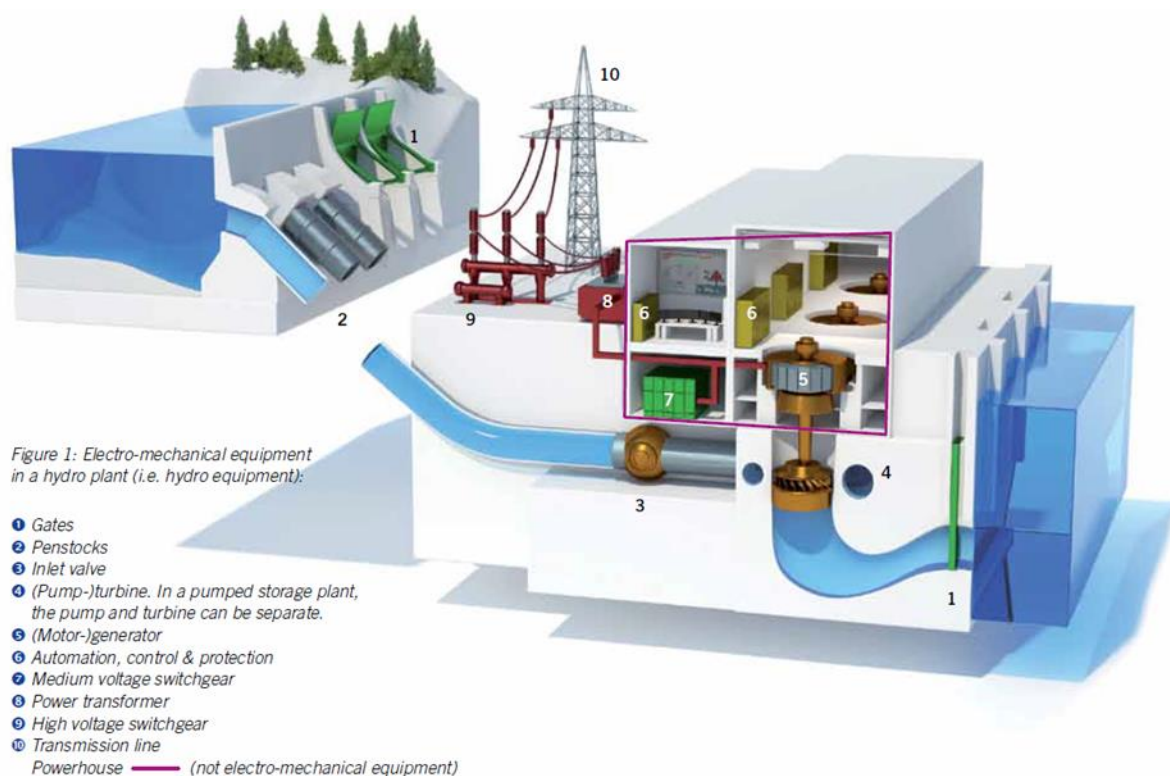
Figure 1 - Electro-mechanical equipment in a hydro plant
