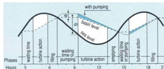
Figure 12-5 – Bi-directional operation
