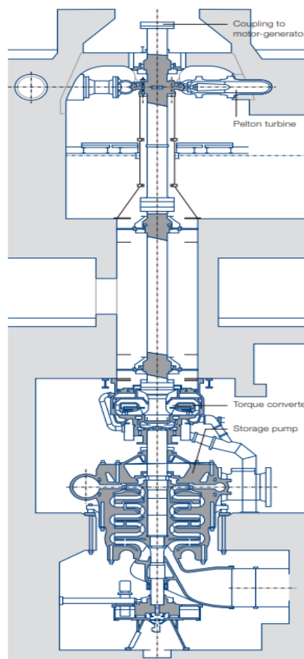
Figure 6-3 - Configuration of a ternary set system
