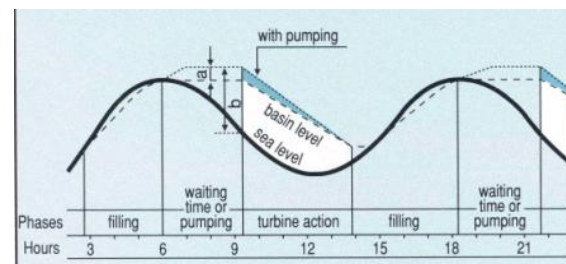
Figure 12-4 - One-directional operation (ebb)
