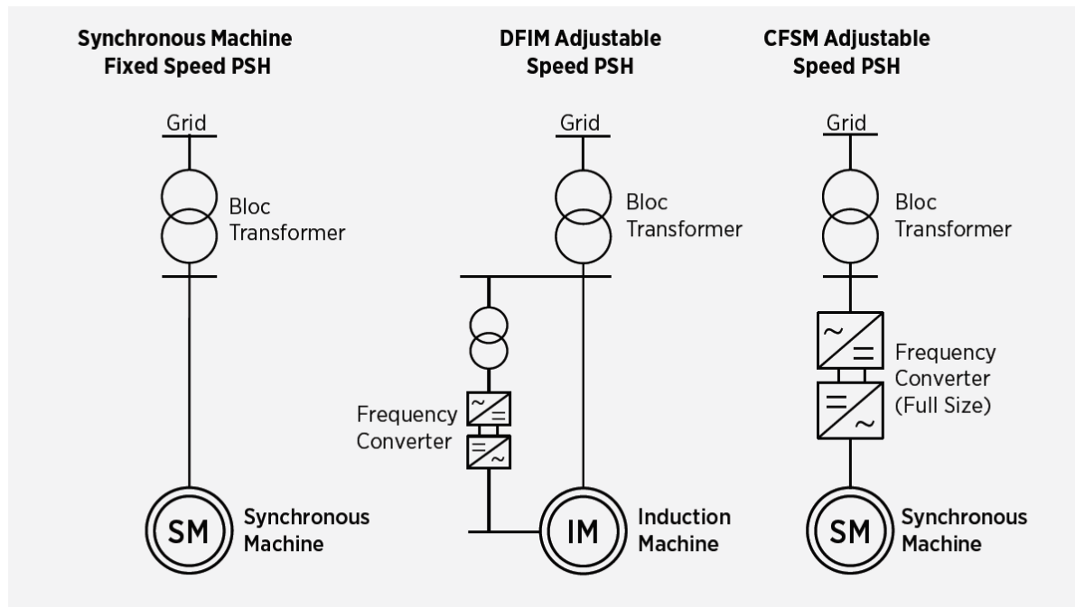
Figure 35: Converter solutions for variable speed operations (Koritarov et al., 2015)
