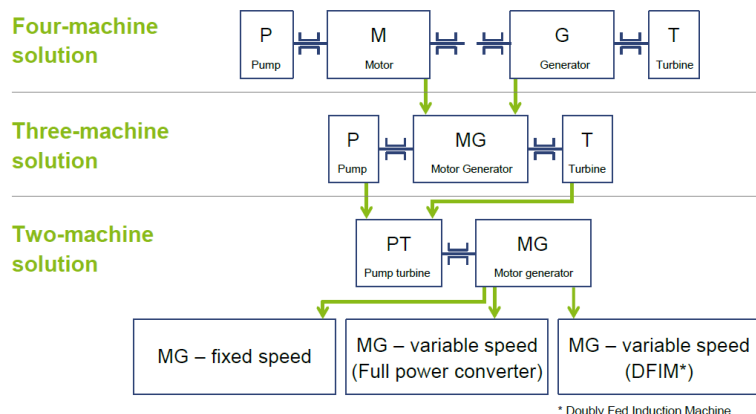
Figure 6-1 - PSP Solutions for balancing services ( Voith)
