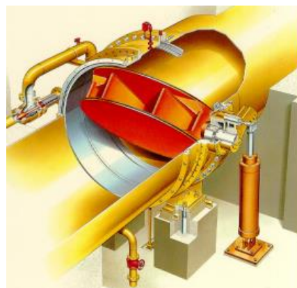
Figure 5-16 – Butterfly valve
