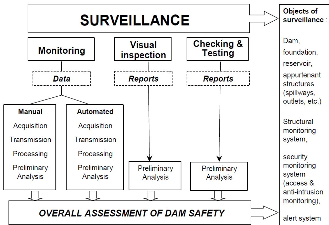
Figure 10-1 – Conceptualisation of dams' surveillance systems
