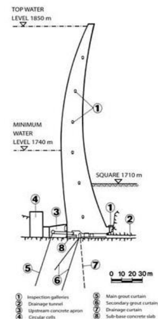
Figure 4-2: Tignes arch dam EDF (left) and typical section of an arch dam (right)
