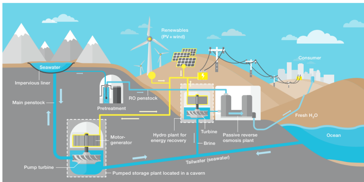
Figure 5 - Exemplification of a hybrid power plant combining seawater pumped storage, plus wind and/or solar power generation, with a desalination (source: Voith)
